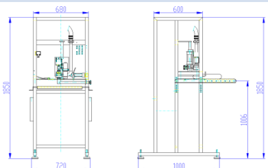
Abmessungen L/B/H: 1200/800/2000
