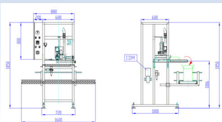
Dimensions L/B/H: 1500/1600/2000
